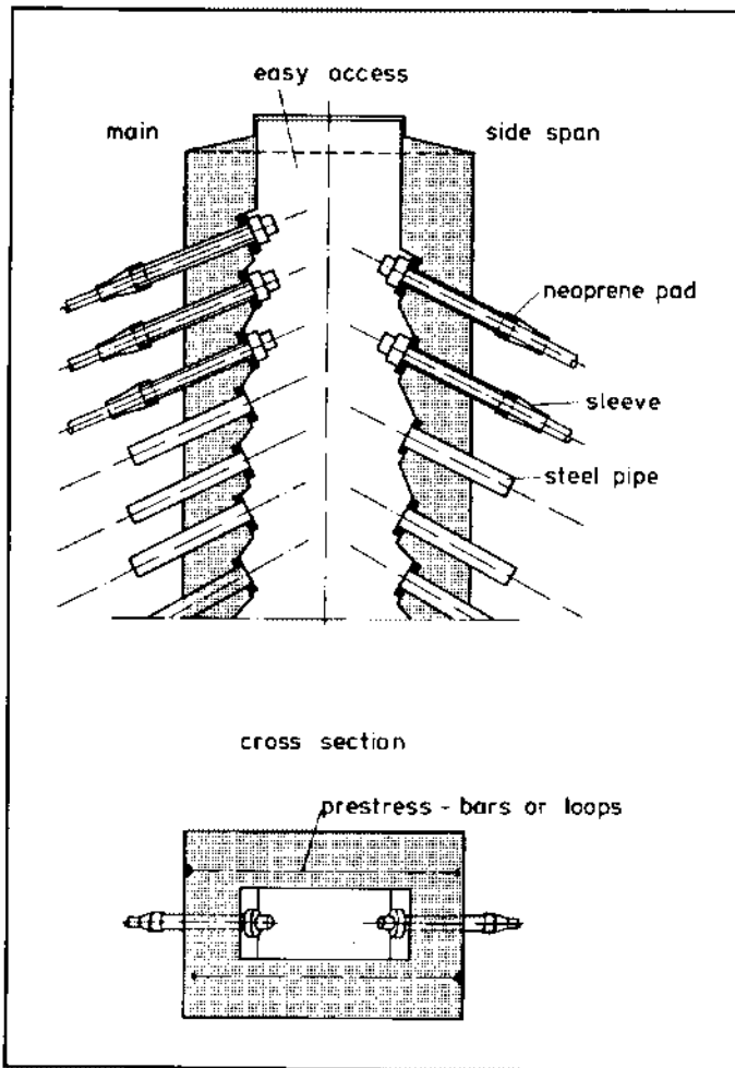
Fig. 40. Cable anchorage inside tower with box section.
