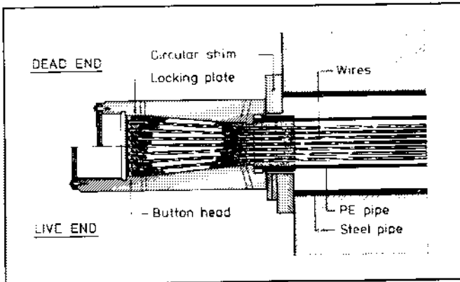
Fig. 35. HIAM anchorage of BBR.
