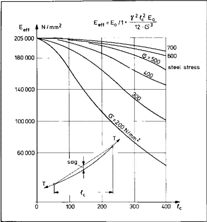
Fig. 5. Effective modulus of elasticity depends primarily on steel stress in cable which in turn affects the cable sag.
