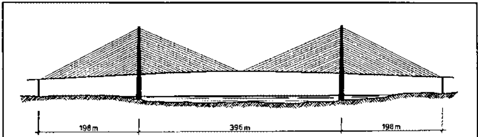
Fig. 10. Dame Point Bridge across St. John's River, Florida, with central expansion joint; design by Ulrich Finsterwalder.
