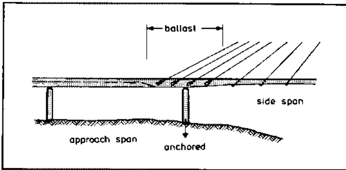
Fig. 33. Continuity to a short approach span avoids large angular changes.
