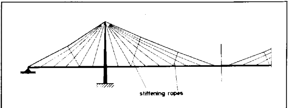
Fig. 6. Stiffening ropes affixed to long cables reduce cable sag.
