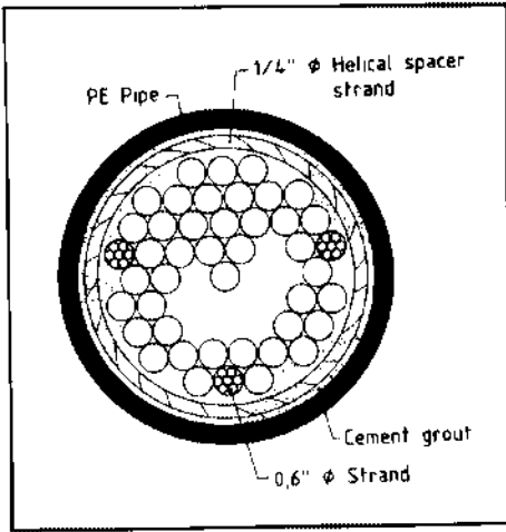
Fig. 34. Section through cable with strands.
