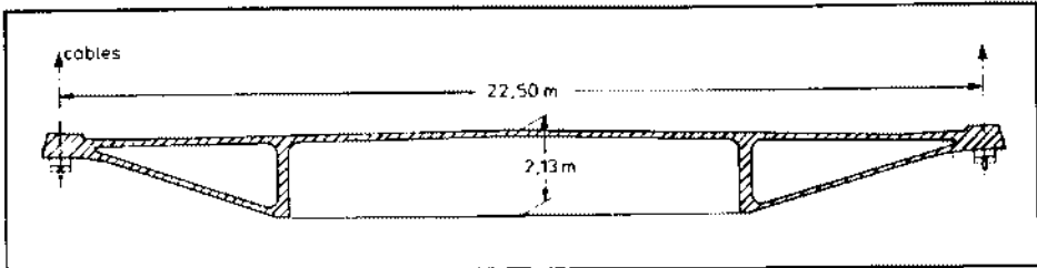
Fig. 23. Cross section of Pasco-Kennewick Bridge (1972), Washington State.
