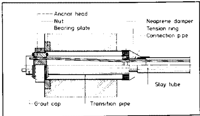
Fig. 36. VSL anchorage for strands.
