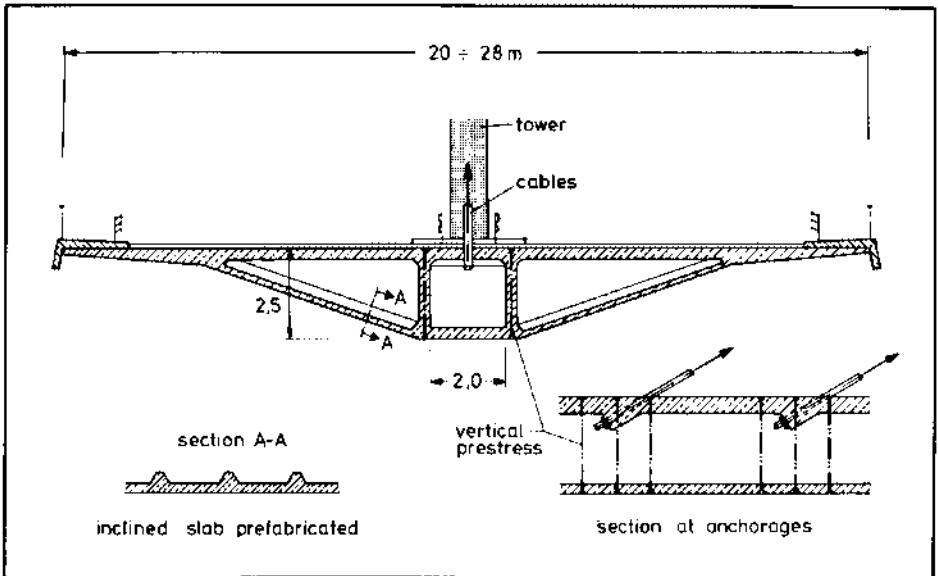
Fig. 29. Stender cross section for cables in the median with simple anchorage (Brotonne Bridge, France).
