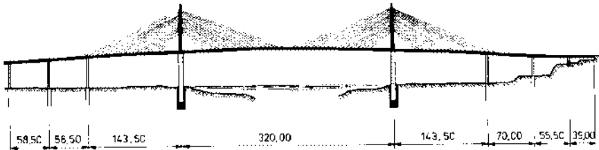
Fig. 11. Semi-fan arrangement of cables leaving a "window" open near the tower; Brotonne Bridge, France.
